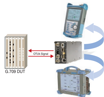
Power Blazer modules support G.709 testing in either the FTB-200 Compact Platform or the FTB-400 Universal Test System.
